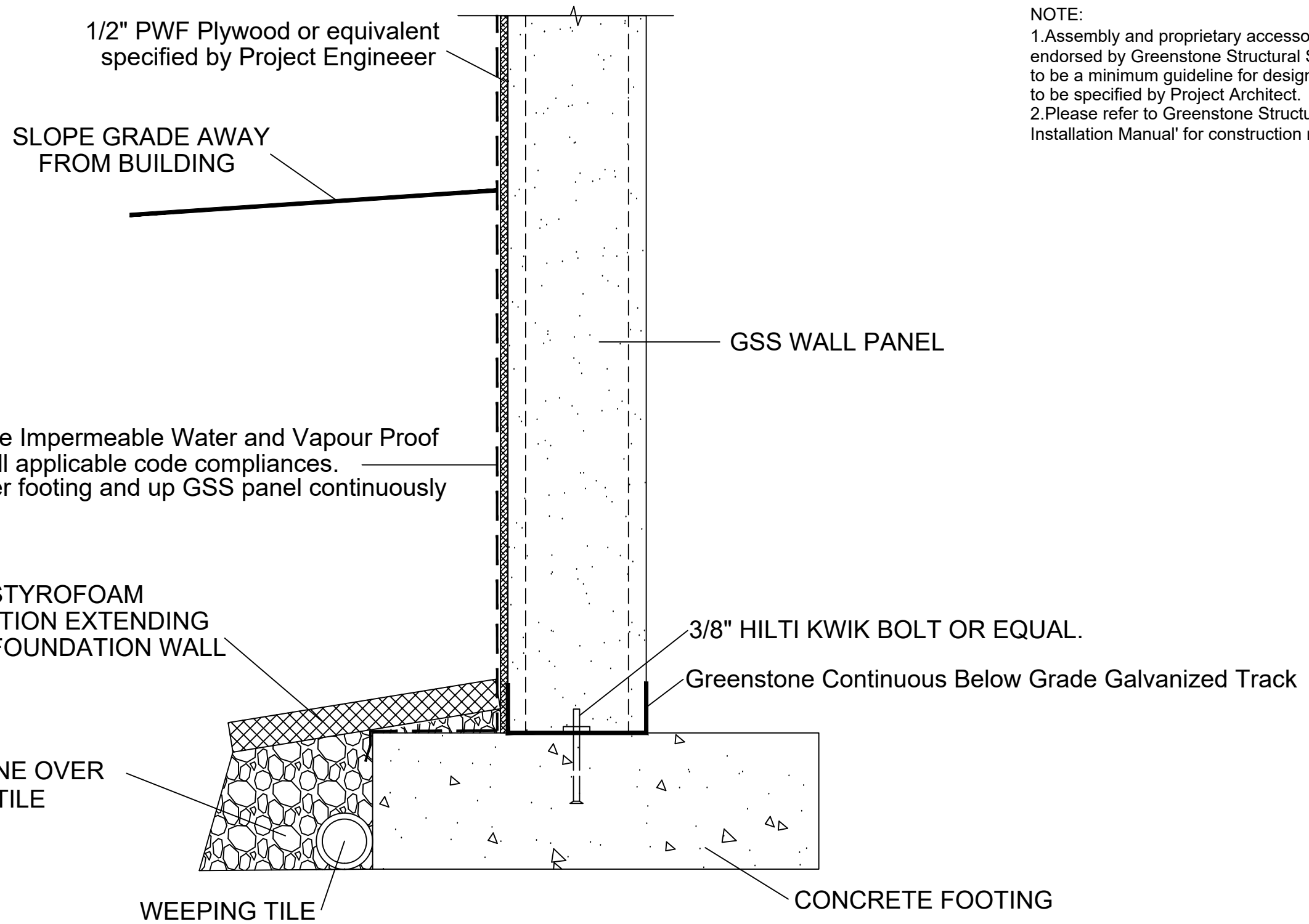
GSS TYP. FOUNDATION DETAIL
